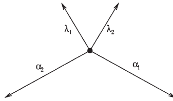
Figure 1. Roots and weights of \mathfrak{sl}(3, \mathbb{C})
